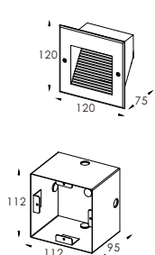
Mounting sleeve
