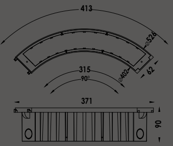
Mounting sleeve
