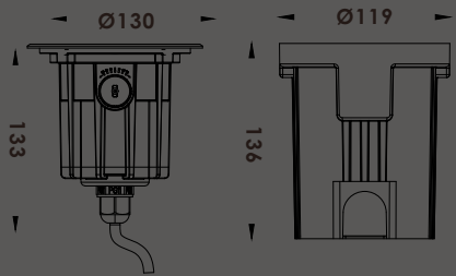
Mounting sleeve
