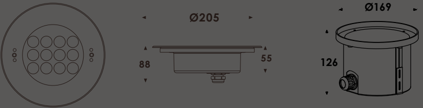
Mounting sleeve
