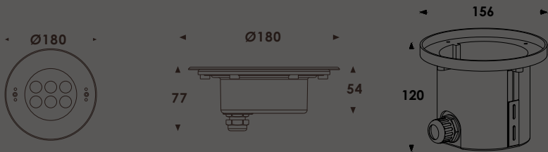
Mounting sleeve
