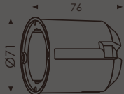
Mounting sleeve
