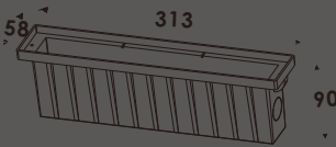
Mounting sleeve
