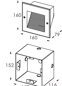
Mounting sleeve
