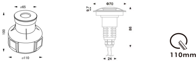
Mounting sleeve
