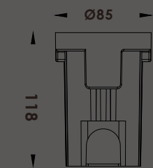
Mounting sleeve
