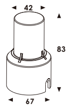
Mounting sleeve
