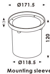
Mounting sleeve
