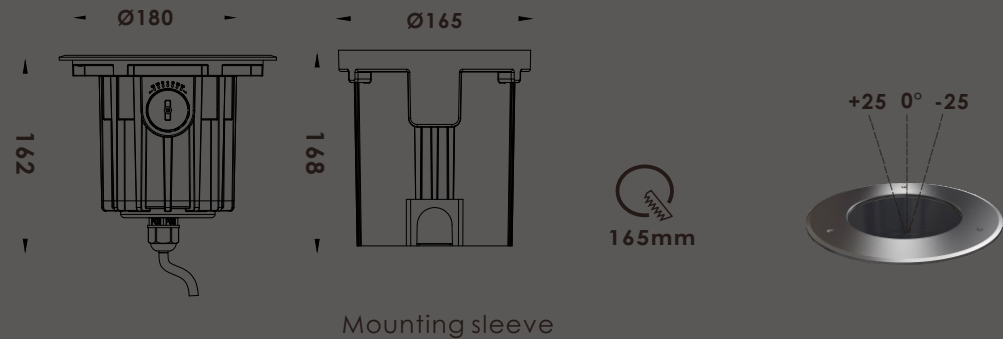
Mounting sleeve
