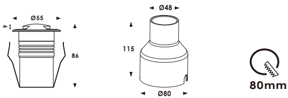
Mounting sleeve
