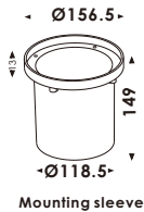
Mounting sleeve
